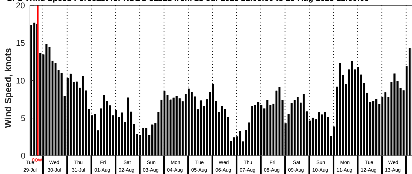
GFS Wind Speed Forecast for NDBC 52211 from 28-Jul-2025 11:00:00 to 13-Aug-2025 11:00:00
