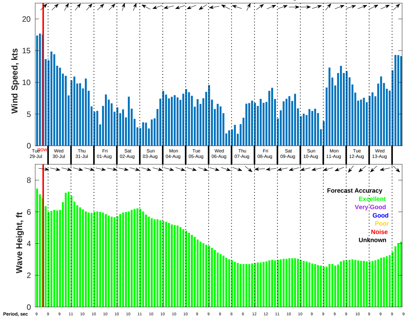
Wind & Wave Forecast for NDBC 52211 from 28-Jul-2025 11:00:00 to 13-Aug-2025 11:00:00
