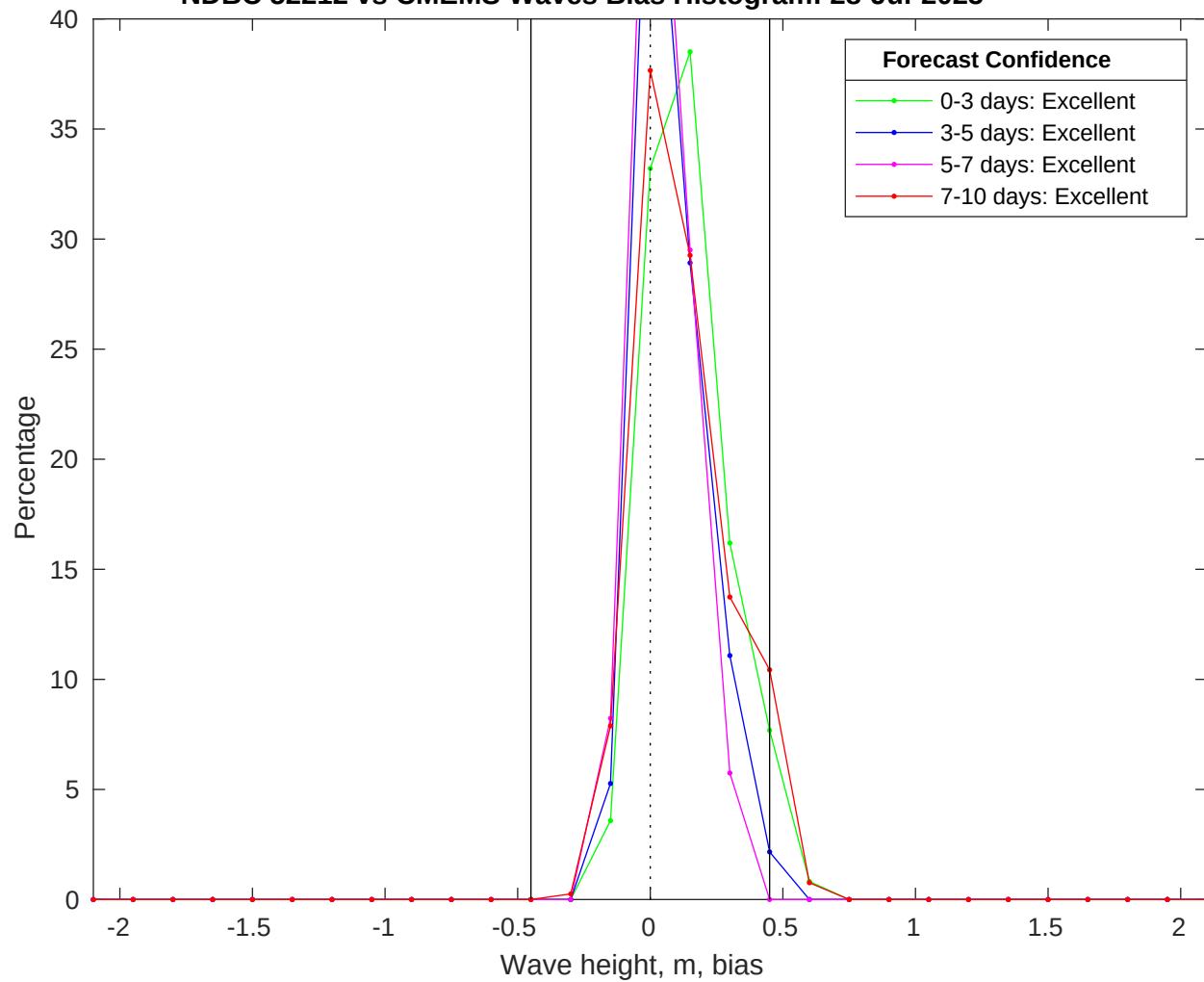
NDBC 52212 vs CMEMS Waves Bias Histogram: 28-Jul-2025
