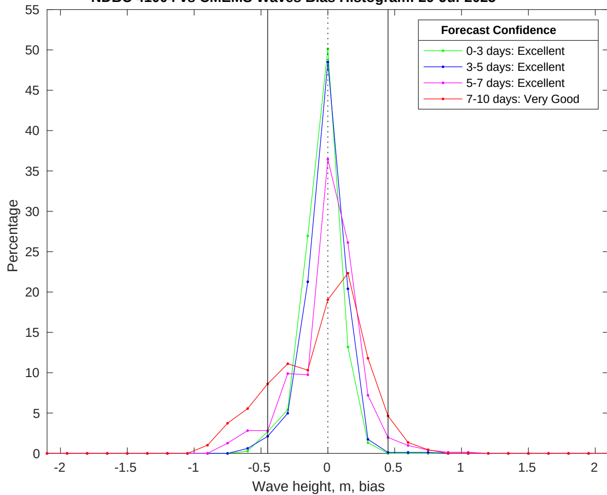
NDBC 41004 vs CMEMS Waves Bias Histogram: 29-Jul-2025
