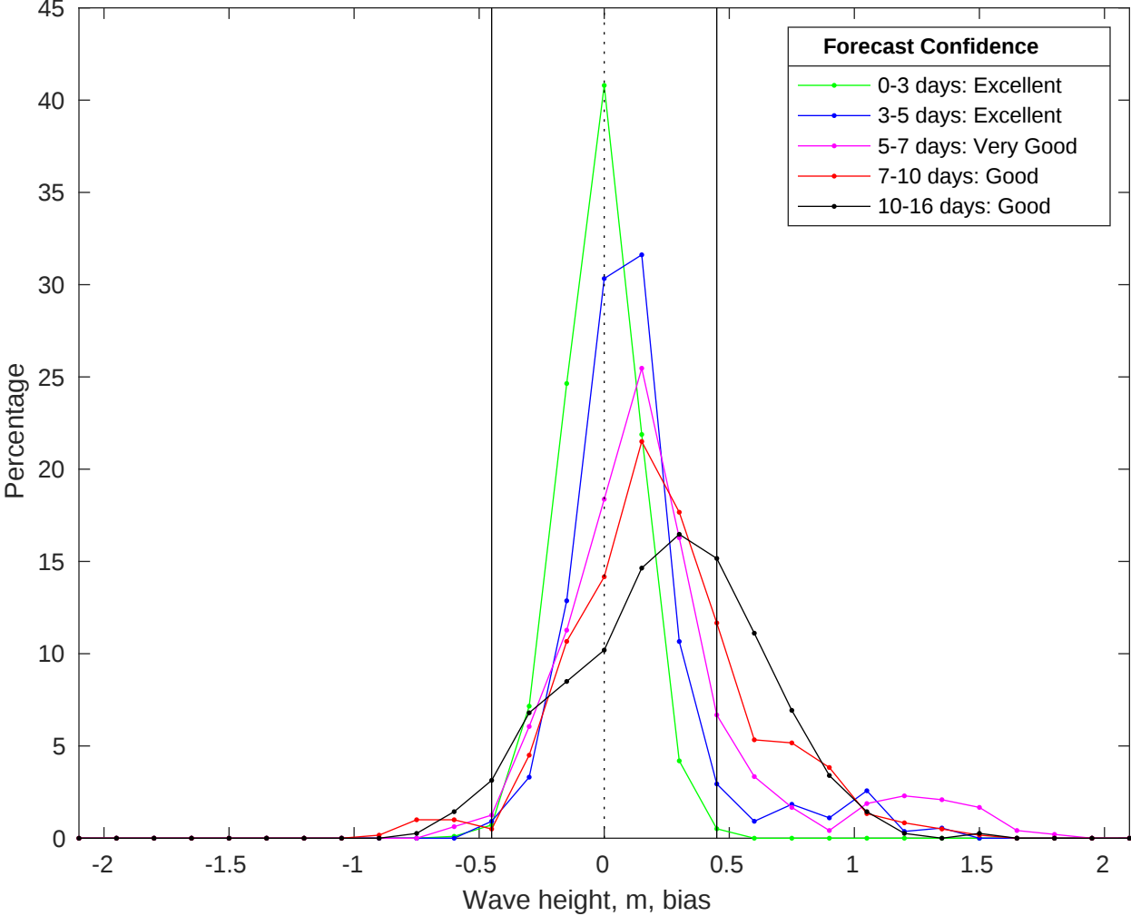
NDBC 41004 vs GFS Waves Bias Histogram: 29-Jul-2025
