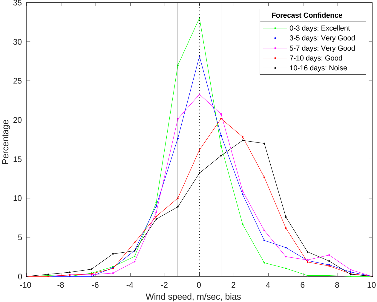
NDBC 41004 vs GFS Winds Bias Histogram: 29-Jul-2025
