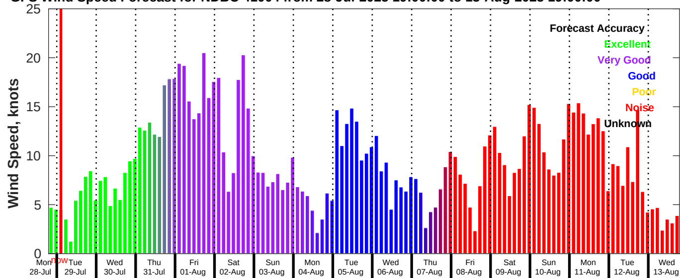
GFS Wind Speed Forecast for NDBC 41004 from 28-Jul-2025 19:00:00 to 13-Aug-2025 19:00:00
