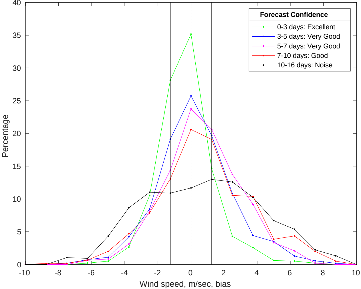
NDBC 41013 vs GFS Winds Bias Histogram: 29-Jul-2025
