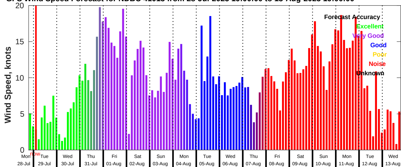
GFS Wind Speed Forecast for NDBC 41013 from 28-Jul-2025 19:00:00 to 13-Aug-2025 19:00:00
