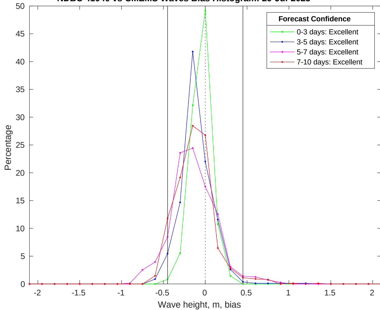
NDBC 41040 vs CMEMS Waves Bias Histogram: 29-Jul-2025
