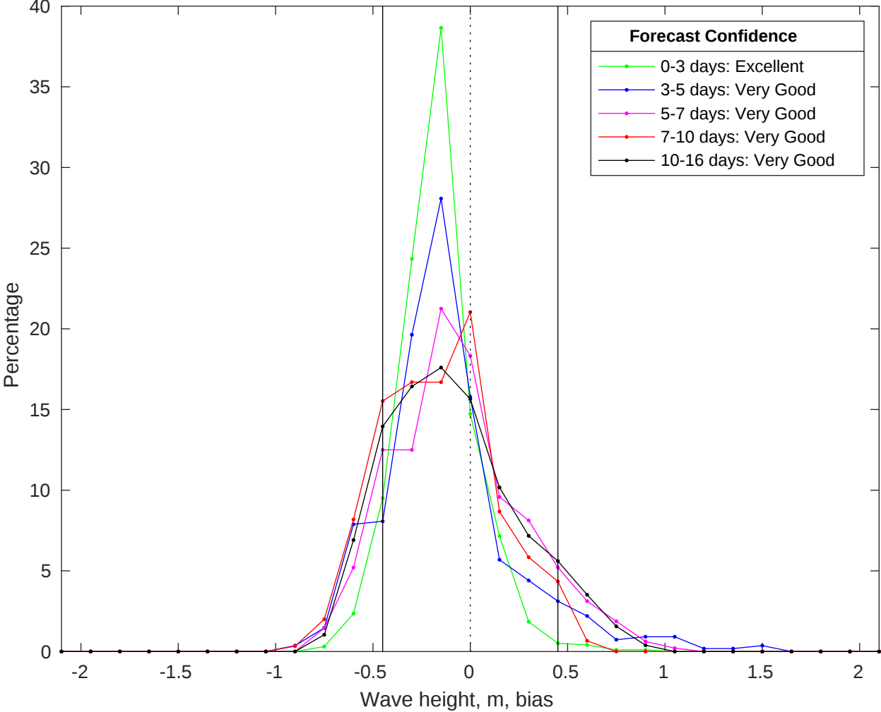
NDBC 41040 vs GFS Waves Bias Histogram: 29-Jul-2025
