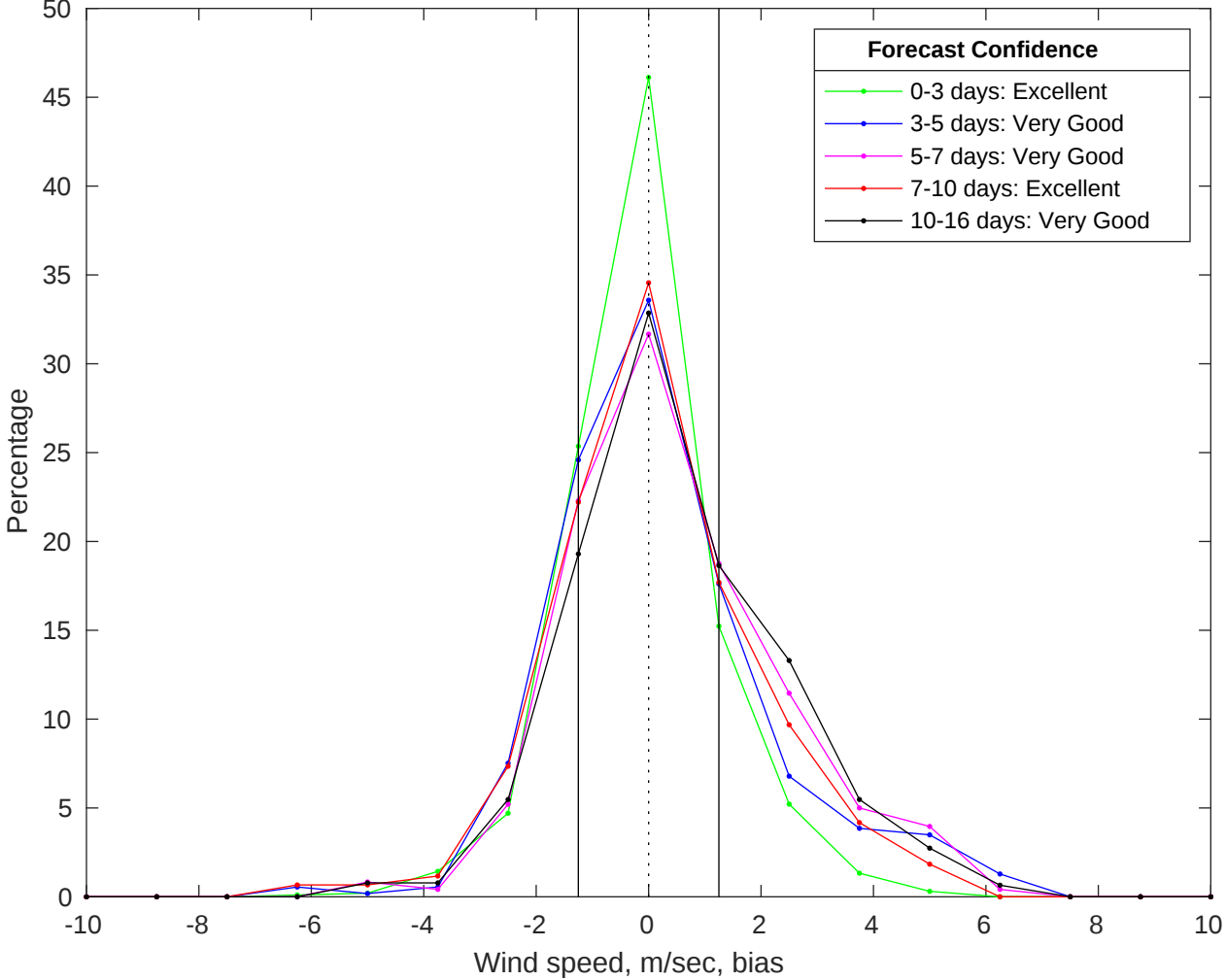
NDBC 41040 vs GFS Winds Bias Histogram: 29-Jul-2025
