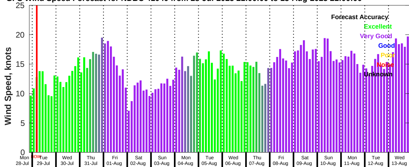
GFS Wind Speed Forecast for NDBC 41040 from 28-Jul-2025 21:00:00 to 13-Aug-2025 21:00:00
