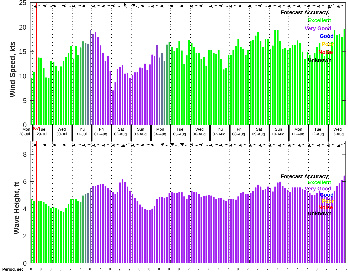
Wind & Wave Forecast for NDBC 41040 from 28-Jul-2025 21:00:00 to 13-Aug-2025 21:00:00
