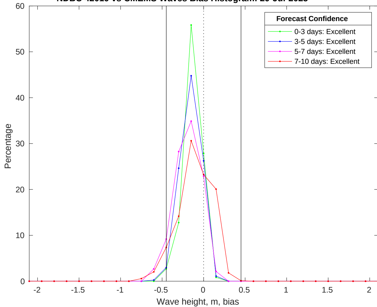
NDBC 42019 vs CMEMS Waves Bias Histogram: 29-Jul-2025
