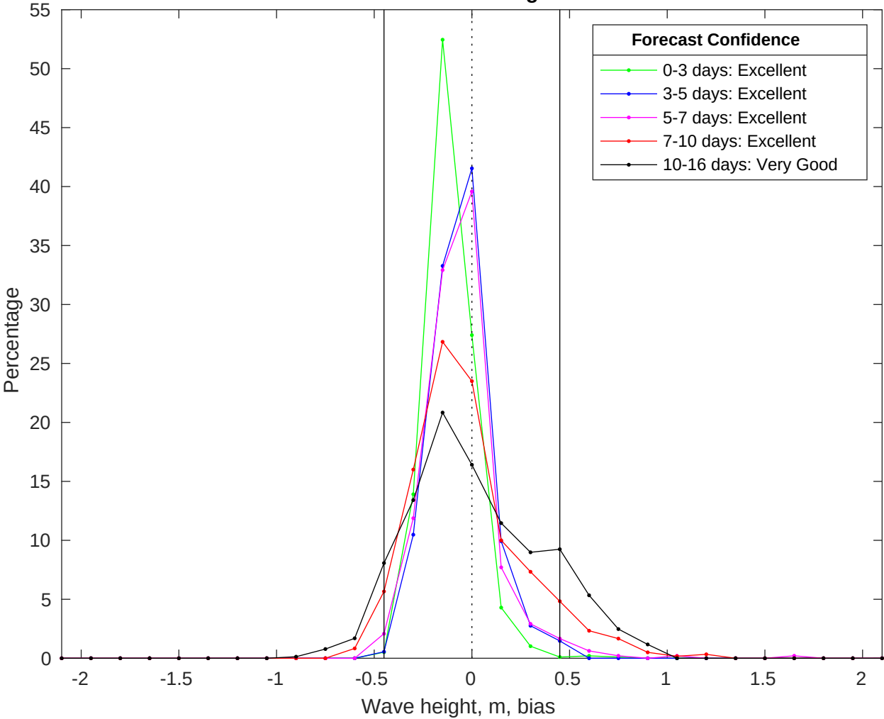
NDBC 42019 vs GFS Waves Bias Histogram: 29-Jul-2025
