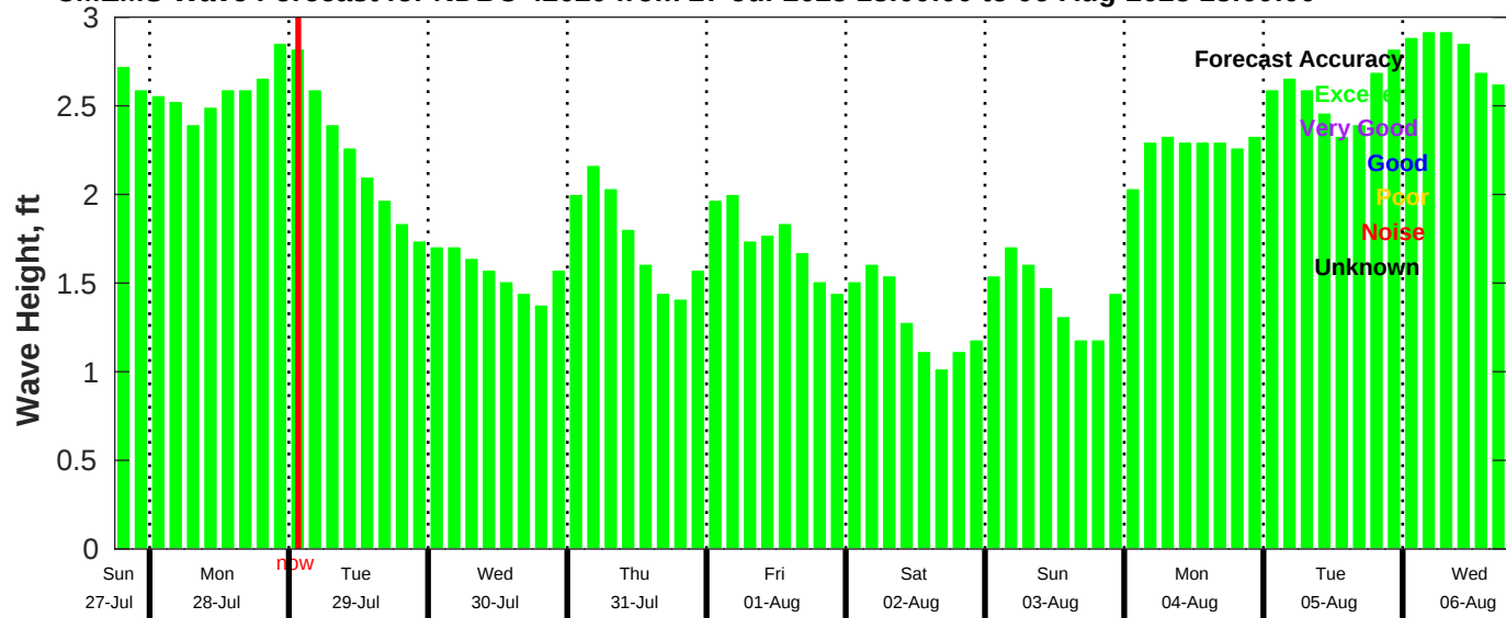
CMEMS Wave Forecast for NDBC 42020 from 27-Jul-2025 18:00:00 to 06-Aug-2025 18:00:00
