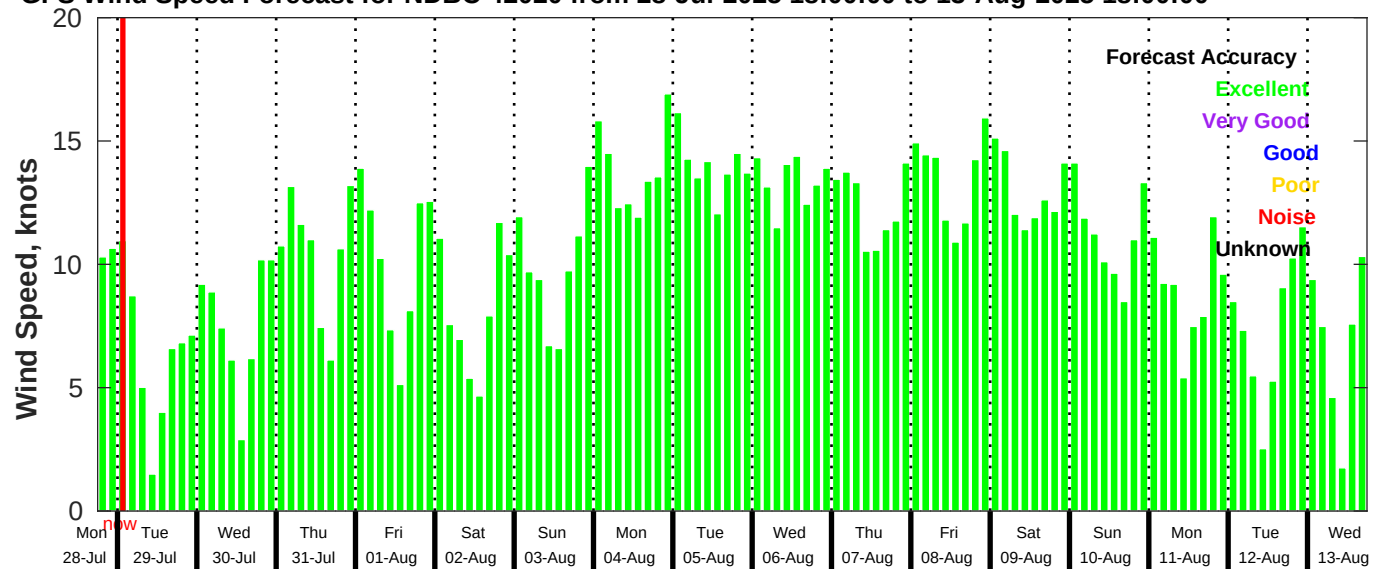
GFS Wind Speed Forecast for NDBC 42020 from 28-Jul-2025 18:00:00 to 13-Aug-2025 18:00:00
