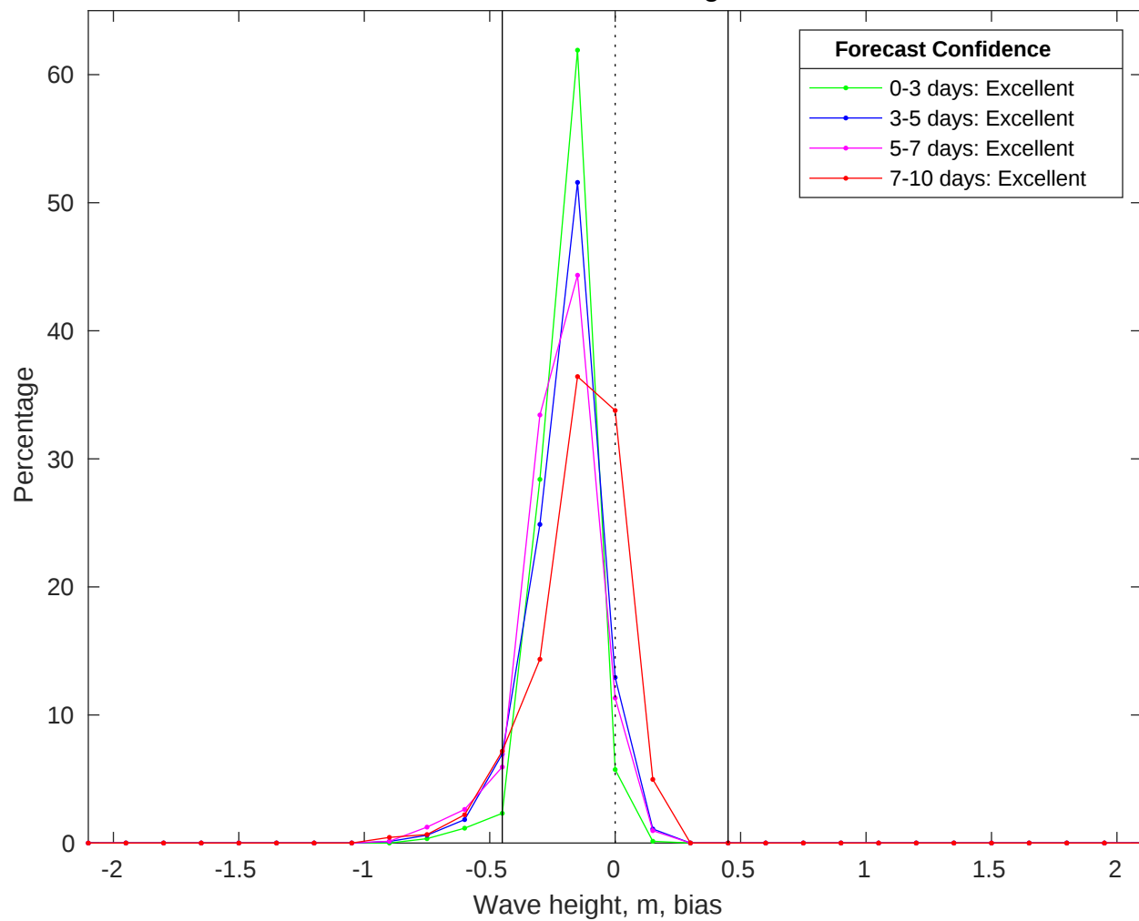
NDBC 42035 vs CMEMS Waves Bias Histogram: 29-Jul-2025
