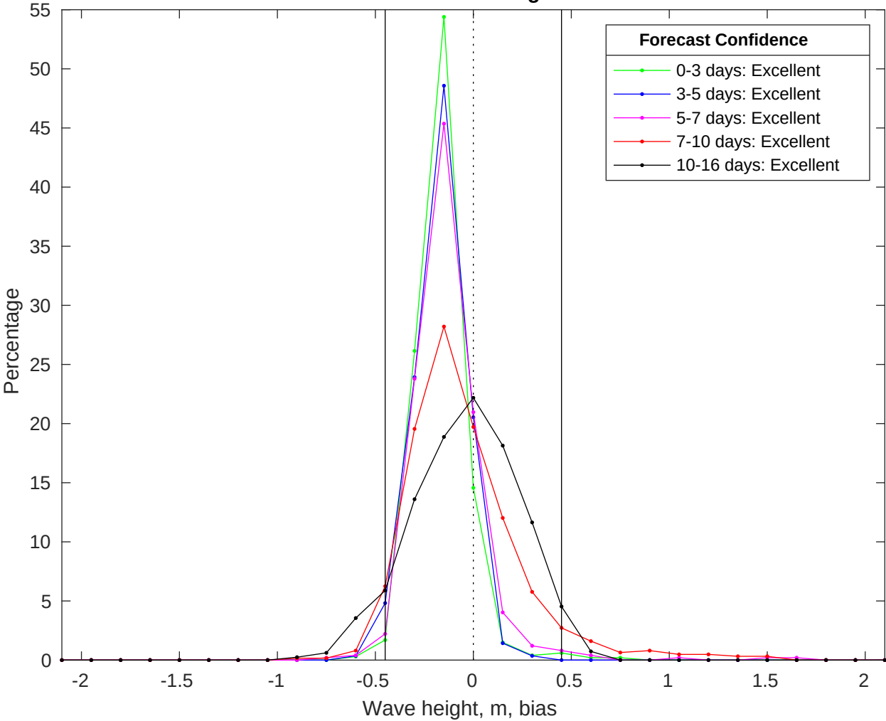
NDBC 42035 vs GFS Waves Bias Histogram: 29-Jul-2025
