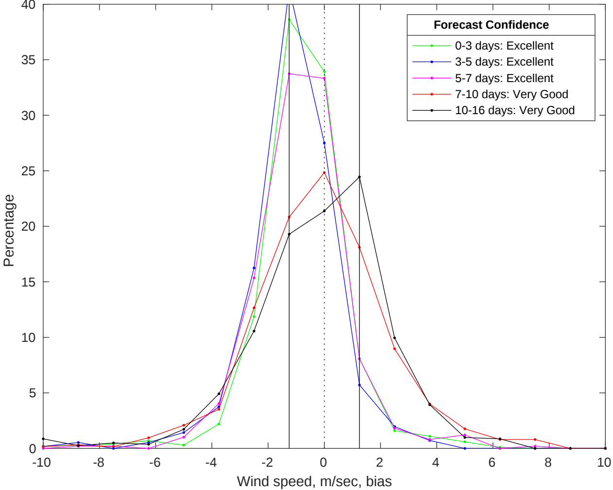
NDBC 42035 vs GFS Winds Bias Histogram: 29-Jul-2025
