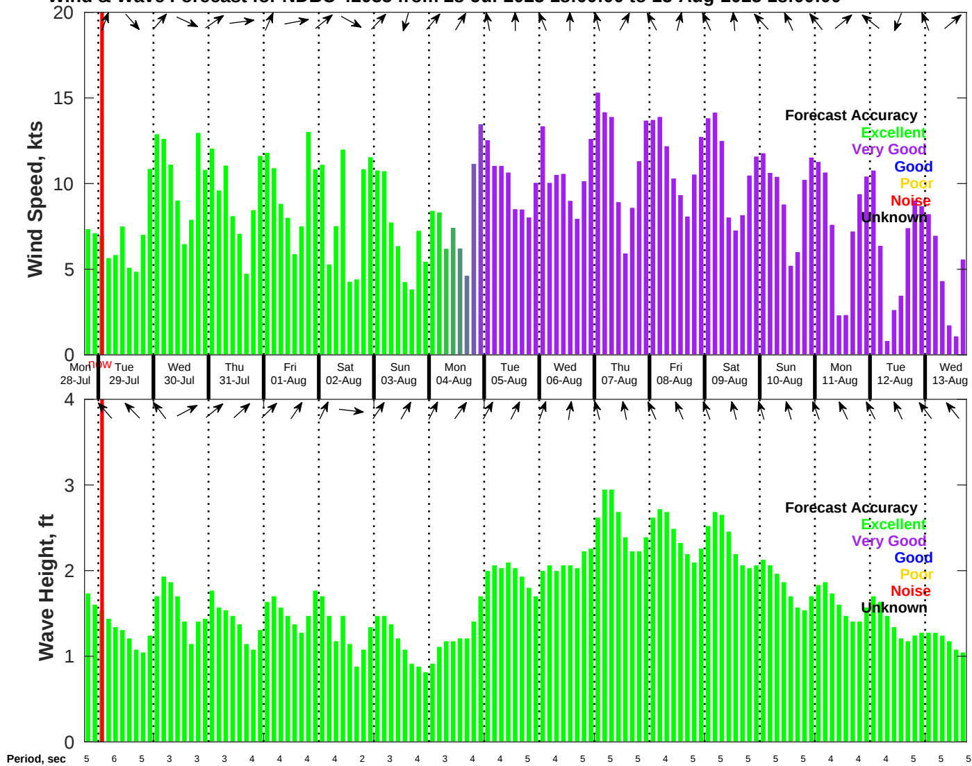
Wind & Wave Forecast for NDBC 42035 from 28-Jul-2025 18:00:00 to 13-Aug-2025 18:00:00
