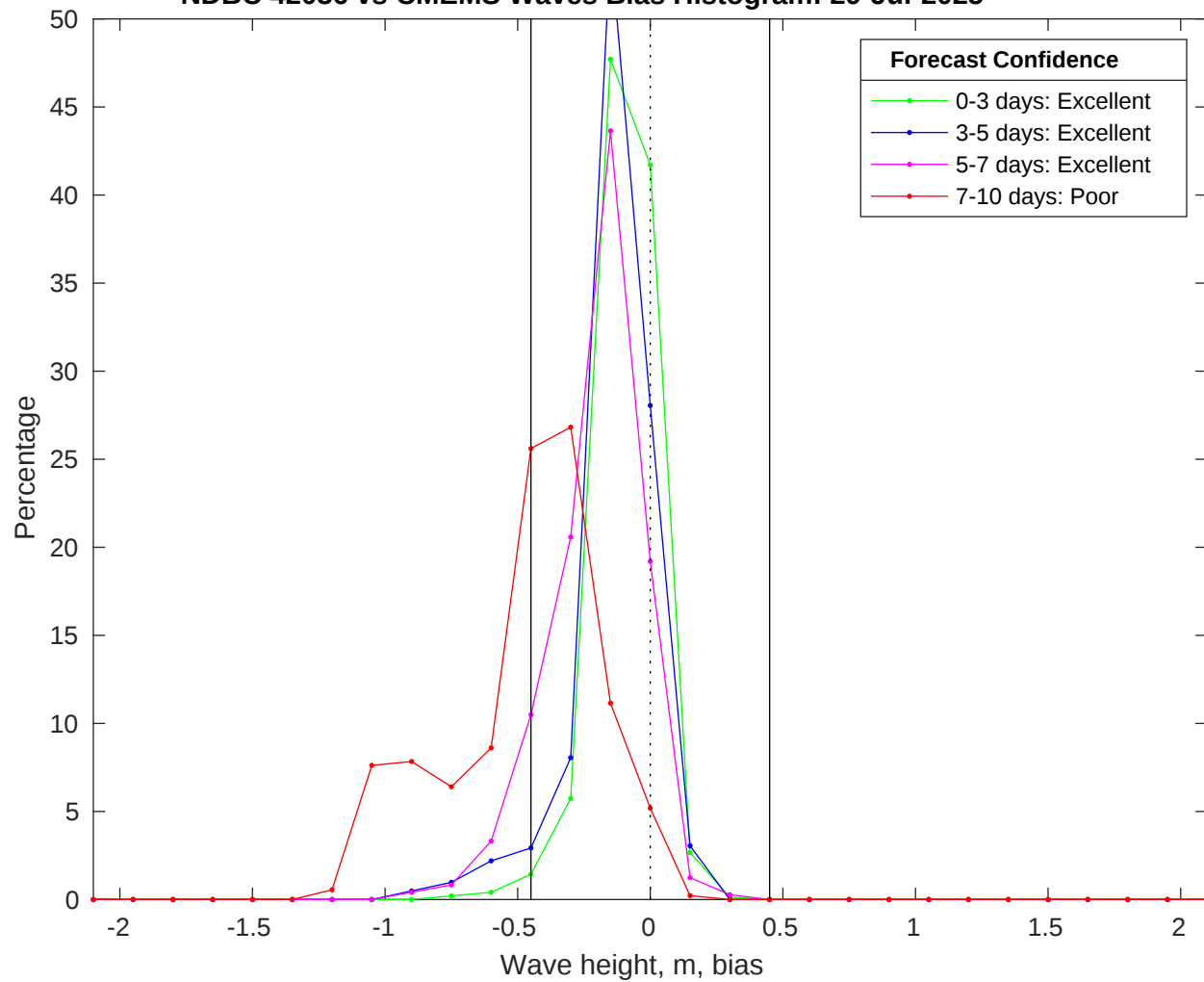
NDBC 42036 vs CMEMS Waves Bias Histogram: 29-Jul-2025
