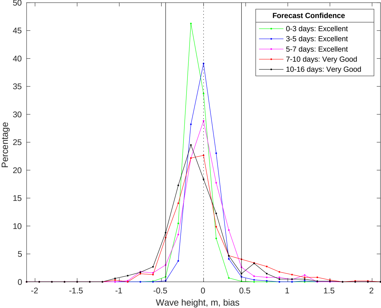
NDBC 42036 vs GFS Waves Bias Histogram: 29-Jul-2025
