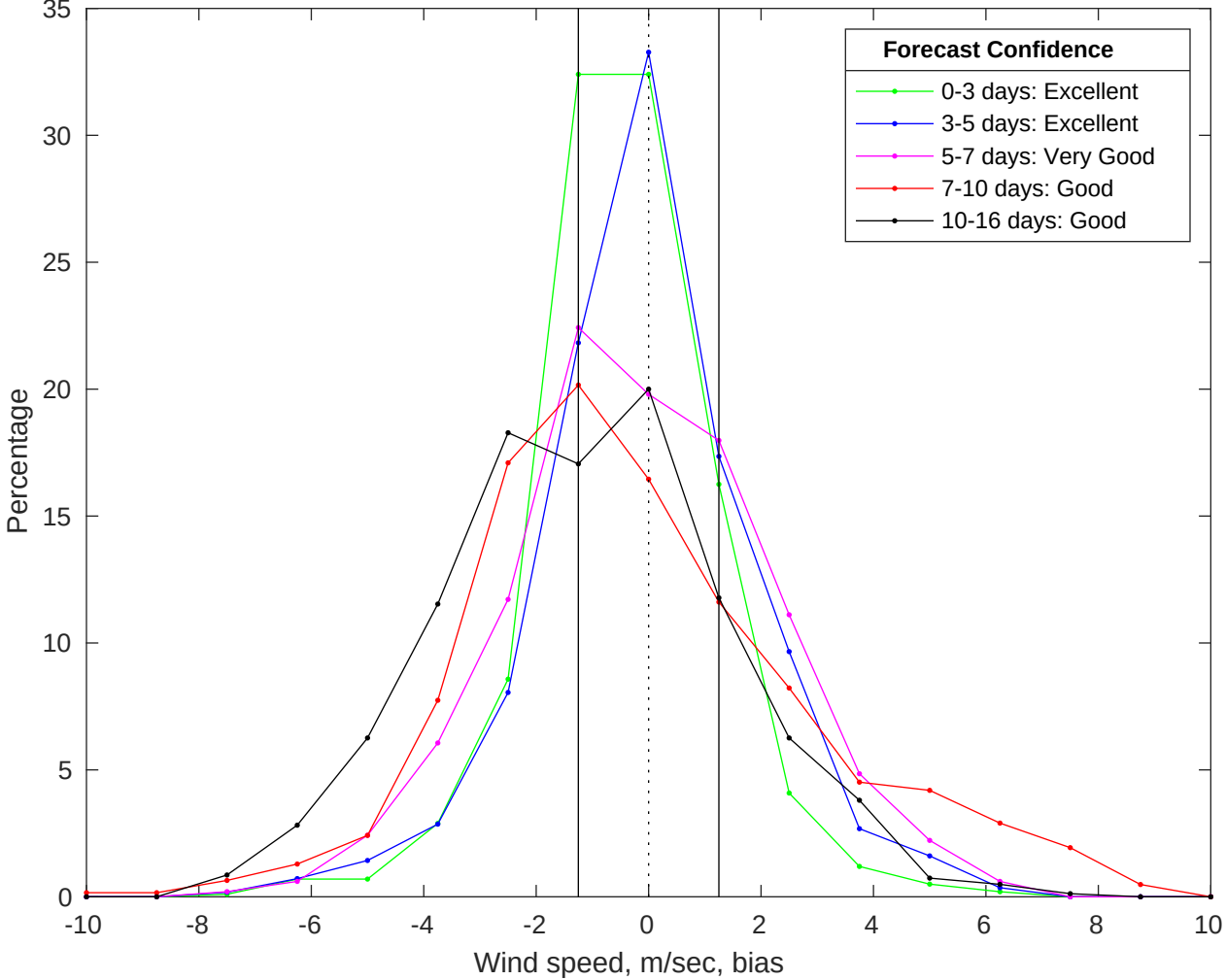
NDBC 42036 vs GFS Winds Bias Histogram: 29-Jul-2025
