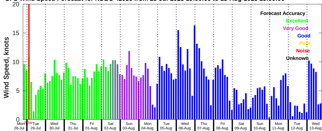
GFS Wind Speed Forecast for NDBC 42036 from 28-Jul-2025 19:00:00 to 13-Aug-2025 19:00:00
