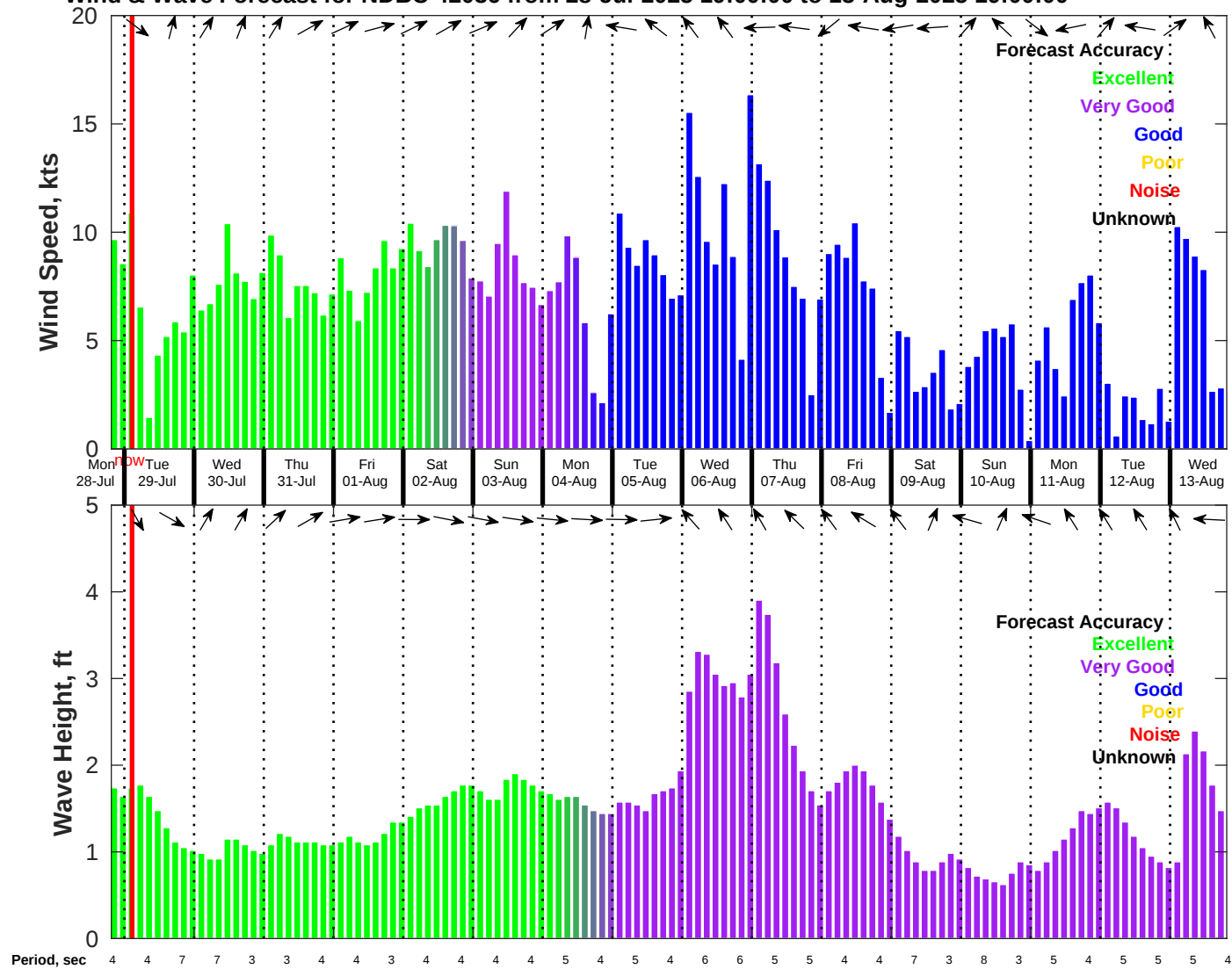
Wind & Wave Forecast for NDBC 42036 from 28-Jul-2025 19:00:00 to 13-Aug-2025 19:00:00
