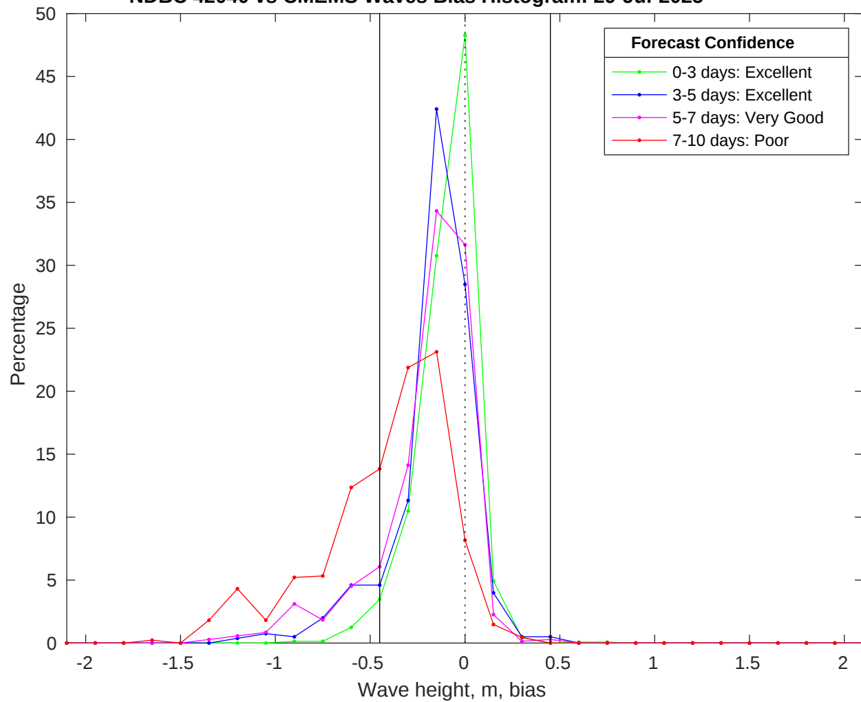
NDBC 42040 vs CMEMS Waves Bias Histogram: 29-Jul-2025
