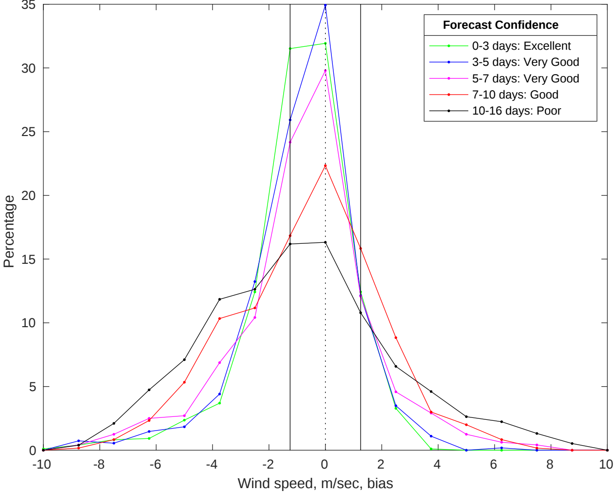
NDBC 42040 vs GFS Winds Bias Histogram: 29-Jul-2025
