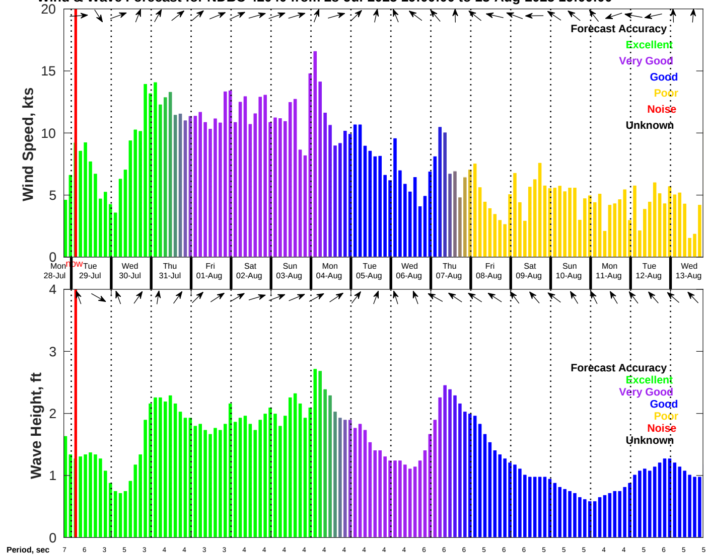
Wind & Wave Forecast for NDBC 42040 from 28-Jul-2025 19:00:00 to 13-Aug-2025 19:00:00
