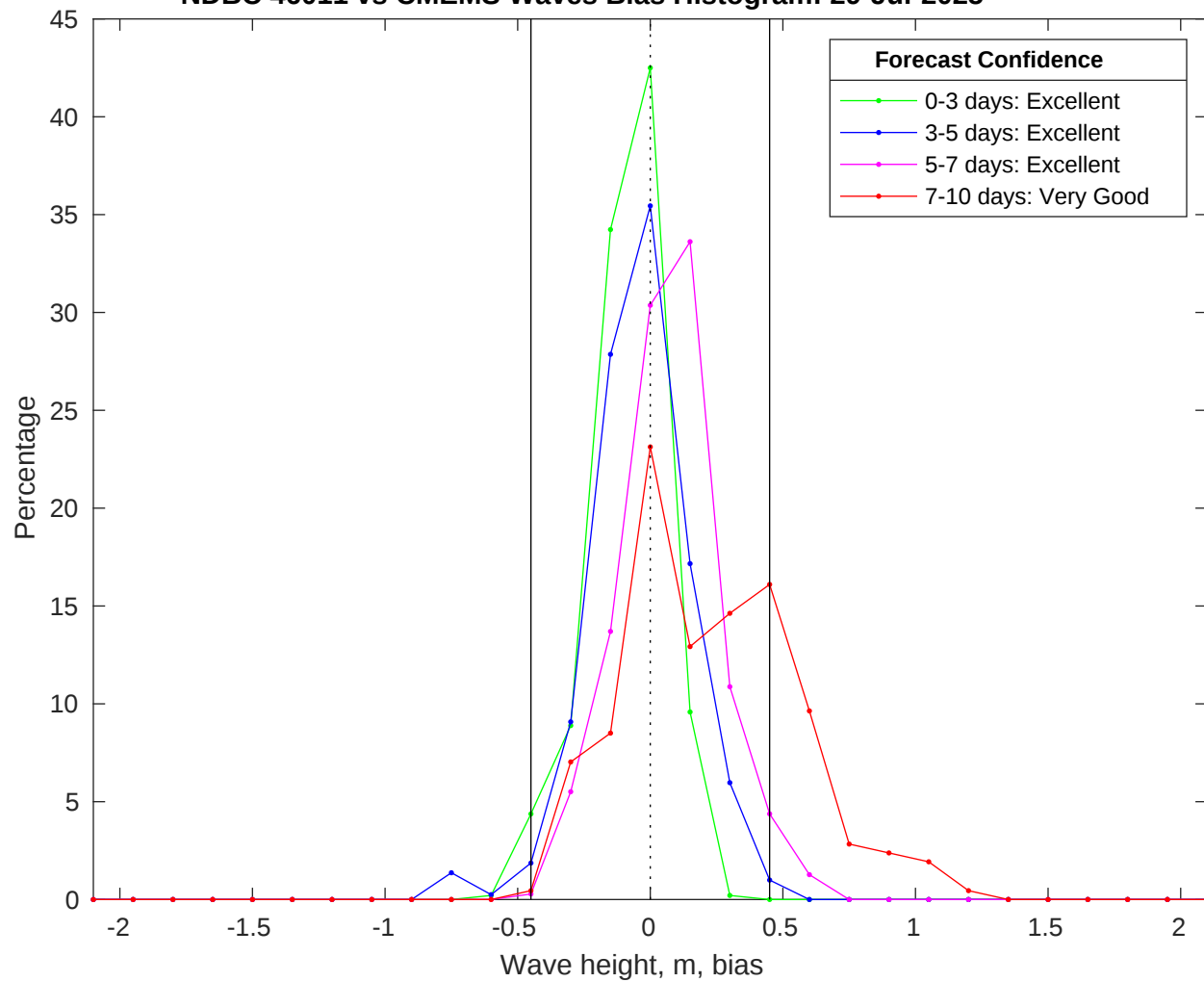
NDBC 46011 vs CMEMS Waves Bias Histogram: 29-Jul-2025
