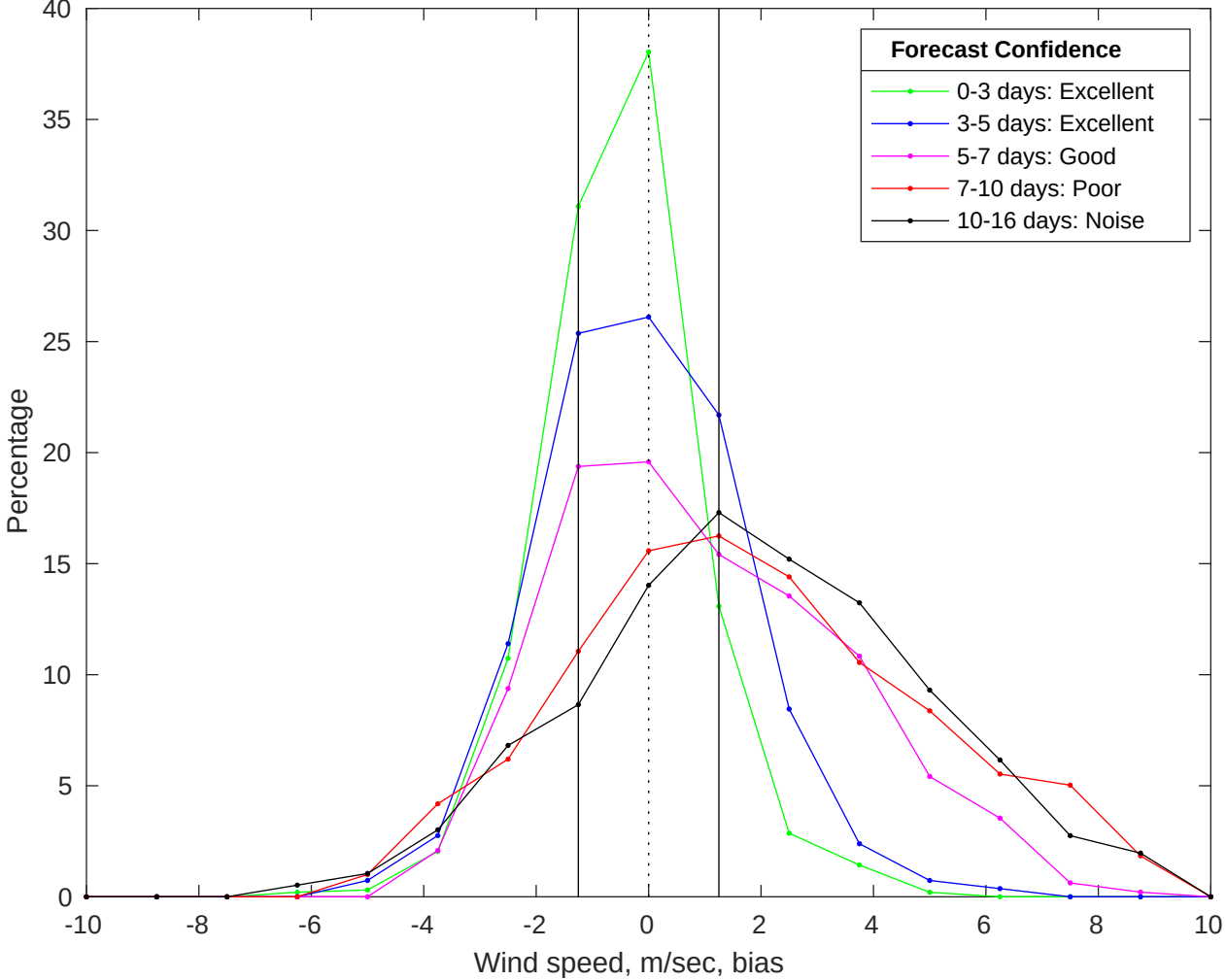
NDBC 46011 vs GFS Winds Bias Histogram: 29-Jul-2025
