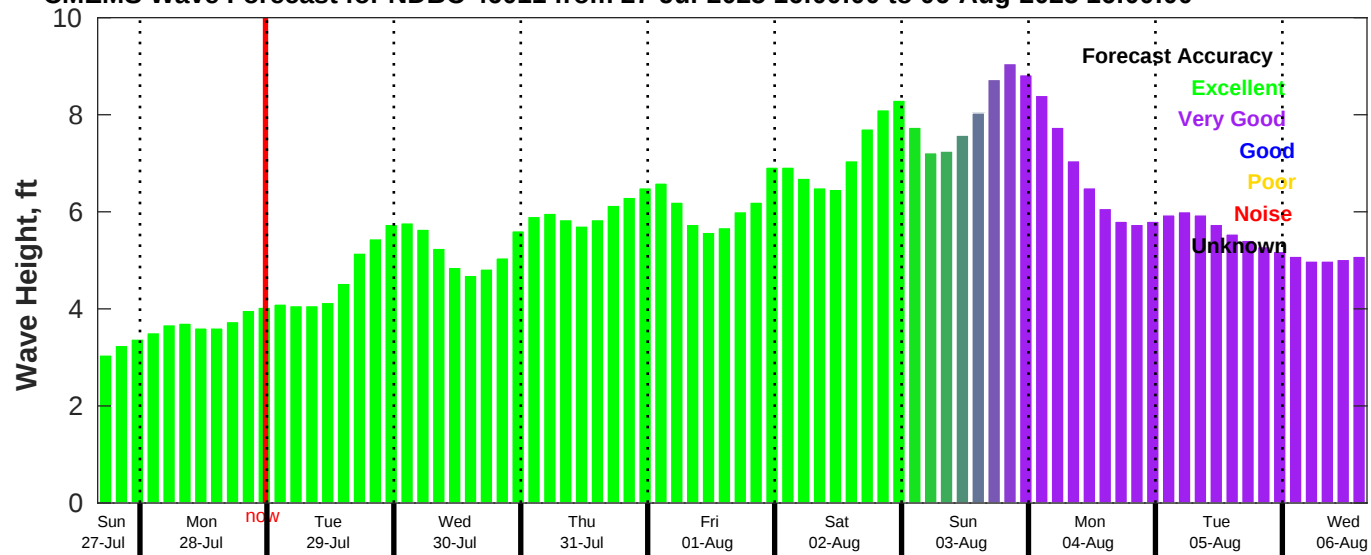
CMEMS Wave Forecast for NDBC 46011 from 27-Jul-2025 16:00:00 to 06-Aug-2025 16:00:00
