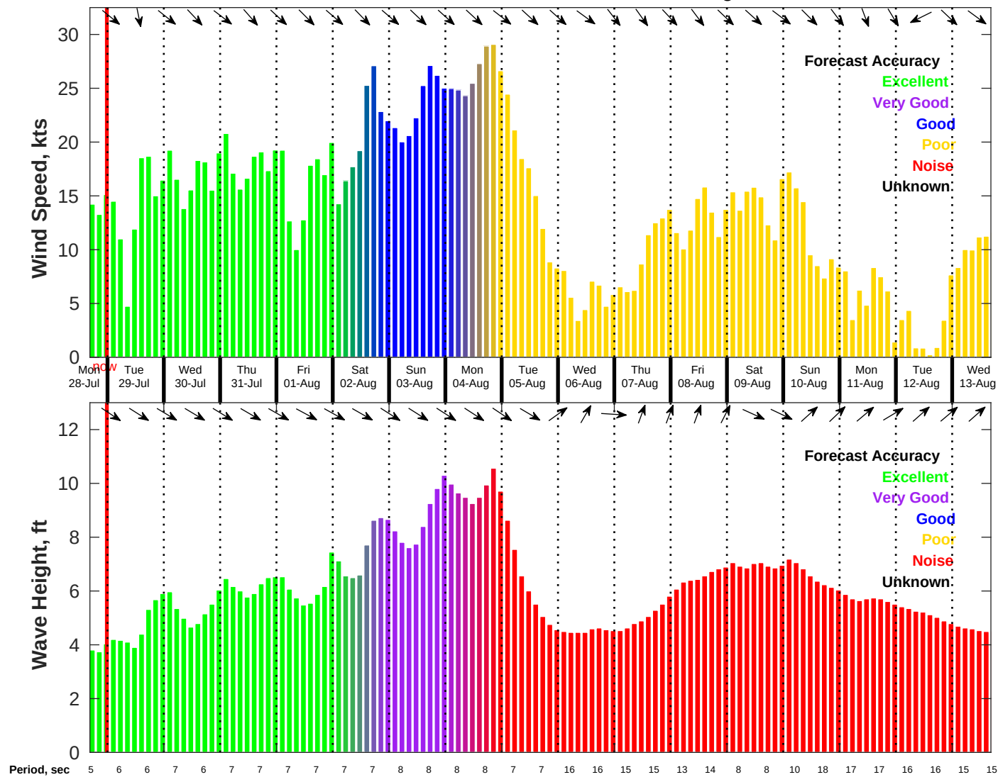
Wind & Wave Forecast for NDBC 46011 from 28-Jul-2025 16:00:00 to 13-Aug-2025 16:00:00
