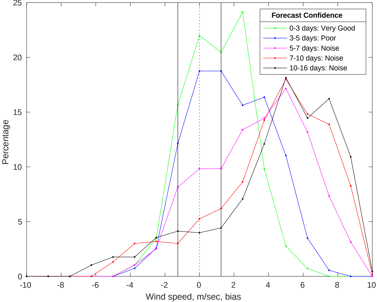
NDBC 46028 vs GFS Winds Bias Histogram: 29-Jul-2025
