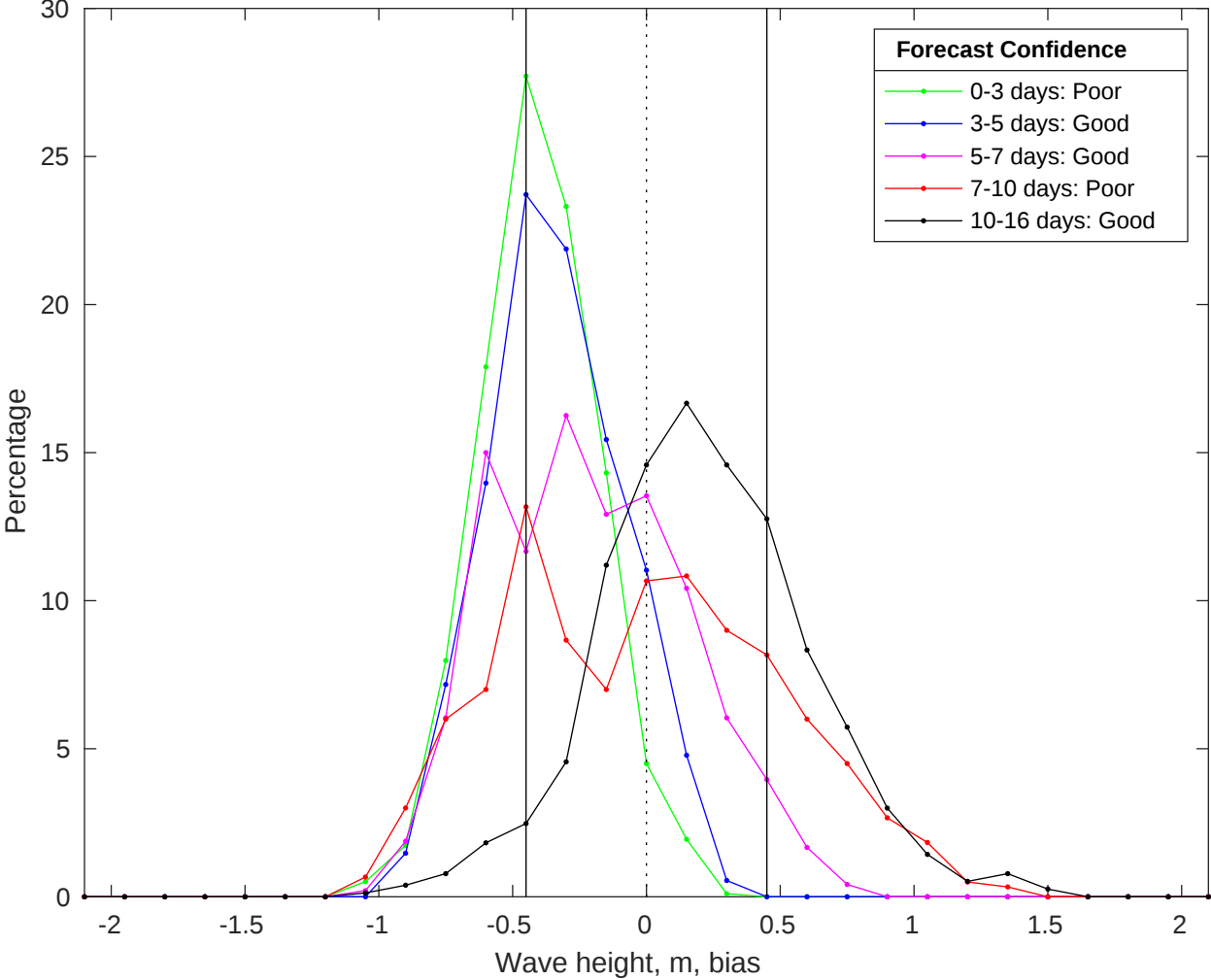
NDBC 46054 vs GFS Waves Bias Histogram: 29-Jul-2025
