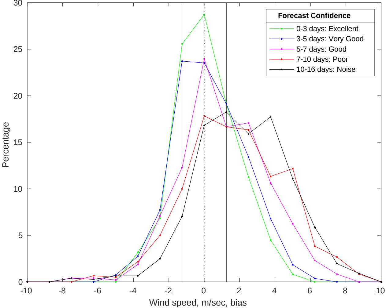
NDBC 46054 vs GFS Winds Bias Histogram: 29-Jul-2025
