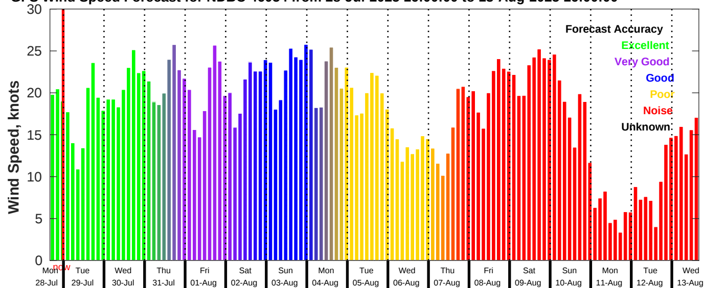
GFS Wind Speed Forecast for NDBC 46054 from 28-Jul-2025 16:00:00 to 13-Aug-2025 16:00:00
