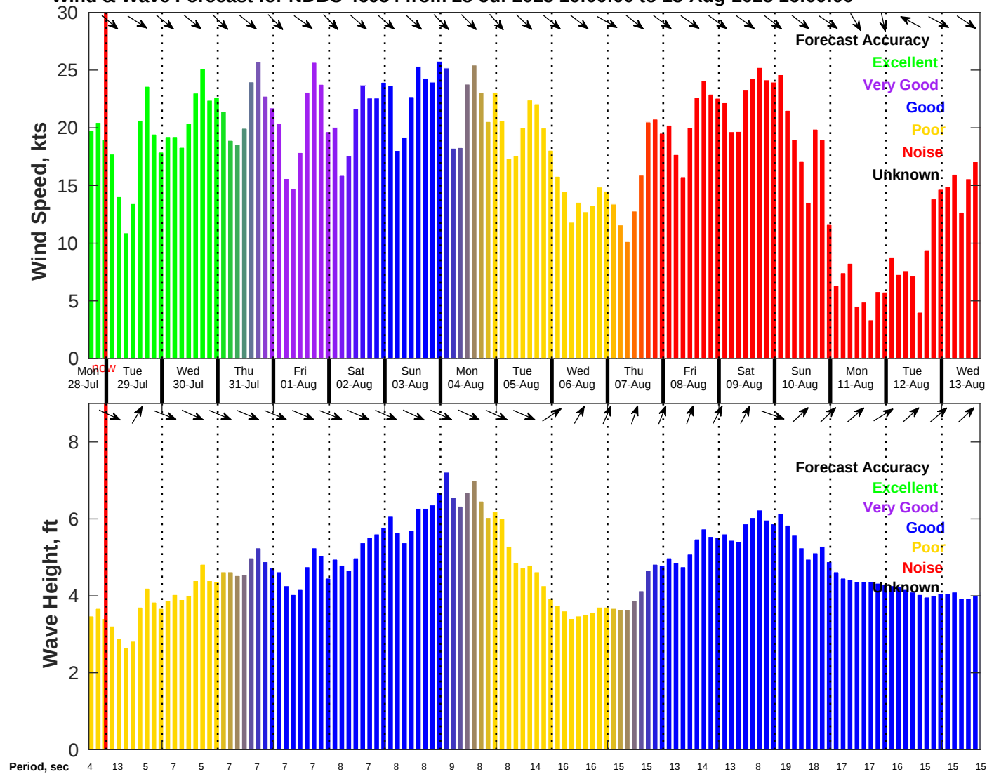
Wind & Wave Forecast for NDBC 46054 from 28-Jul-2025 16:00:00 to 13-Aug-2025 16:00:00
