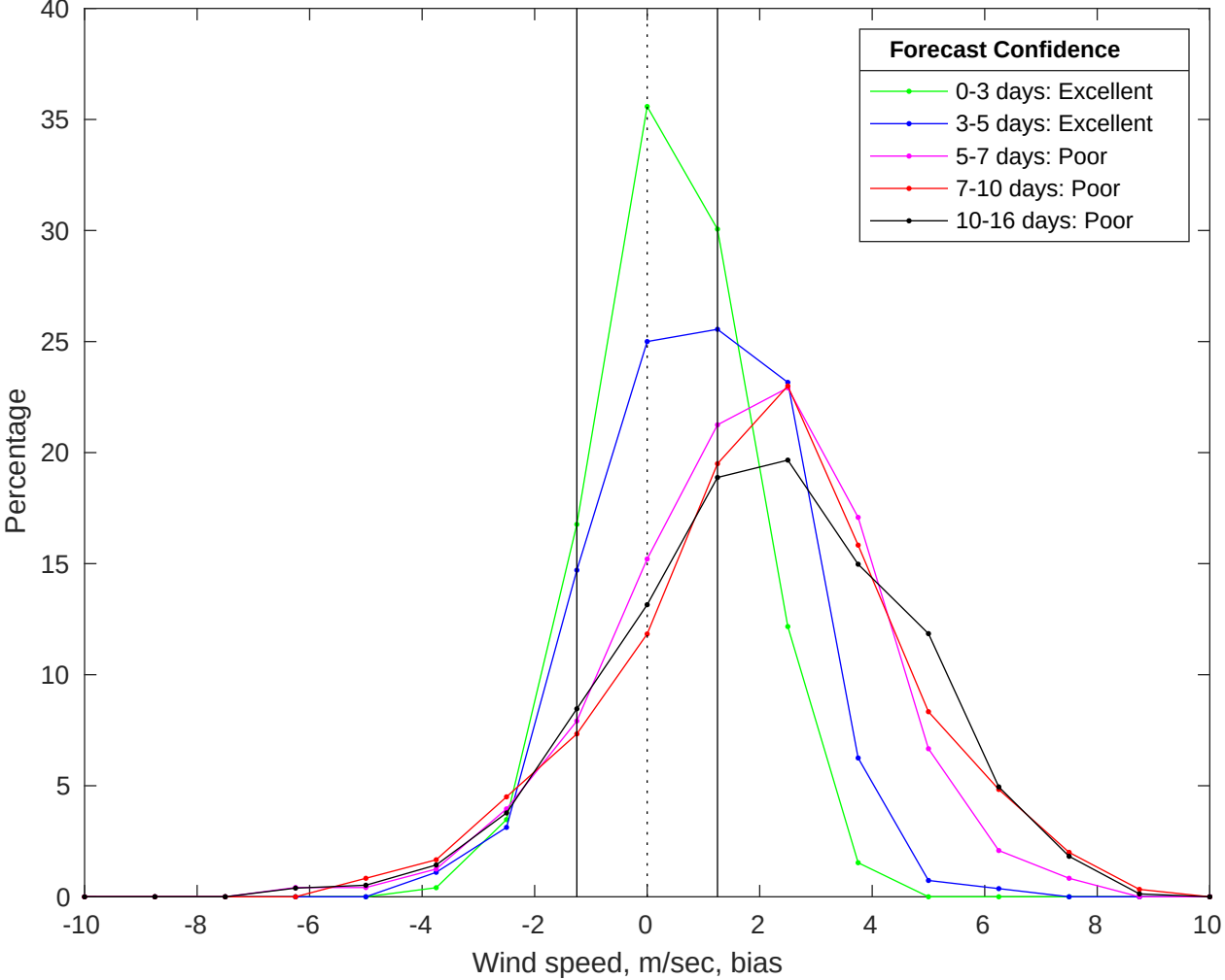
NDBC 46069 vs GFS Winds Bias Histogram: 29-Jul-2025
