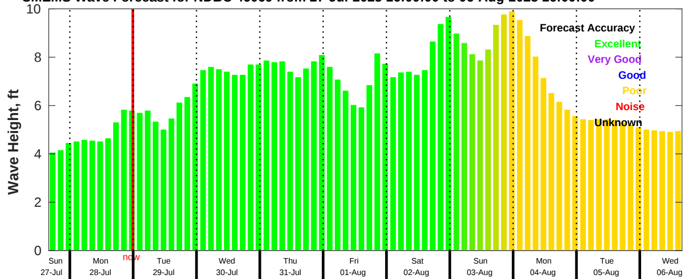
CMEMS Wave Forecast for NDBC 46069 from 27-Jul-2025 16:00:00 to 06-Aug-2025 16:00:00
