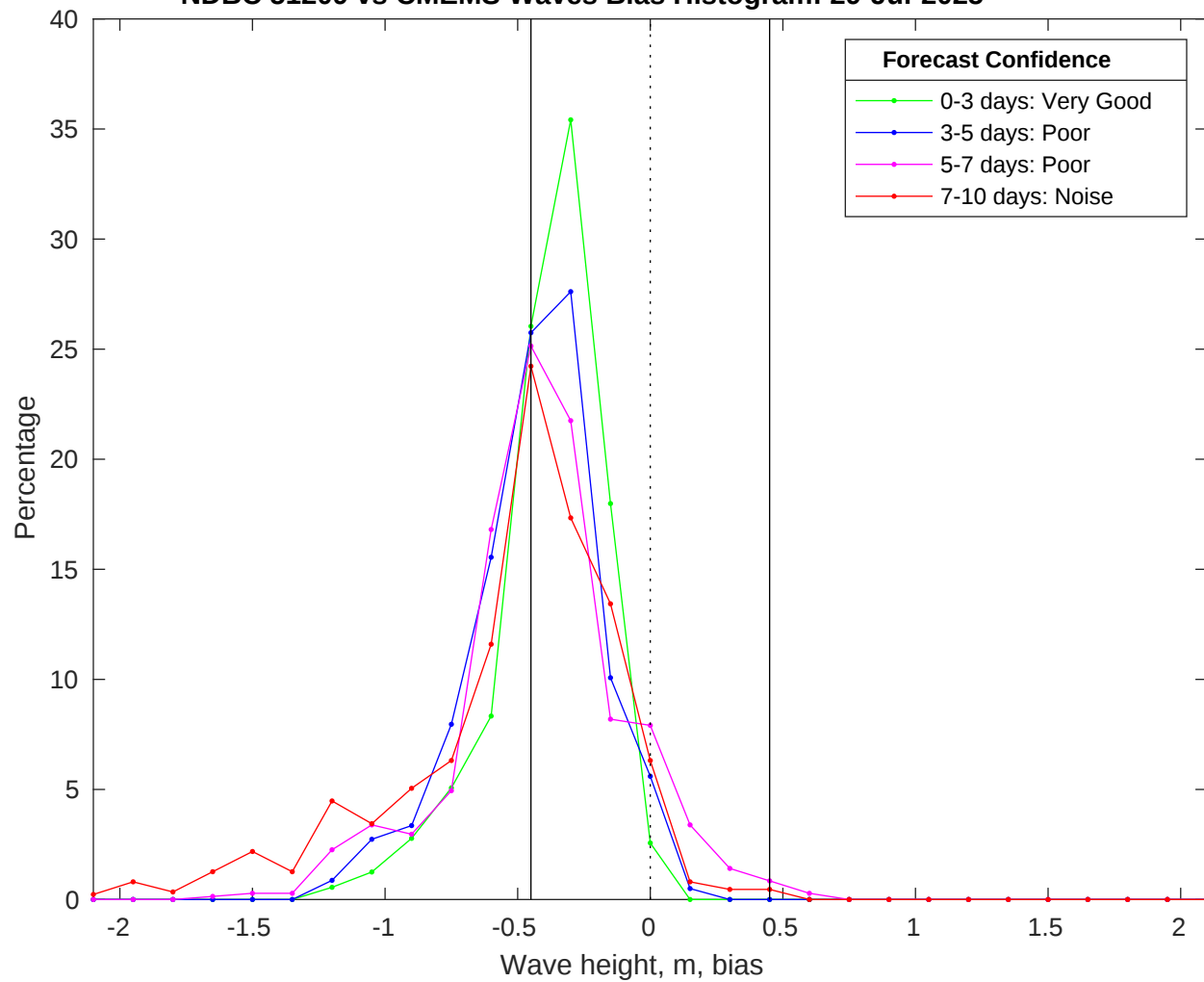
NDBC 51209 vs CMEMS Waves Bias Histogram: 29-Jul-2025
