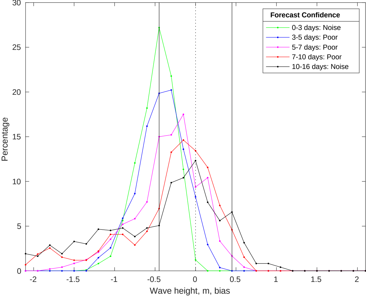
NDBC 51209 vs GFS Waves Bias Histogram: 29-Jul-2025
