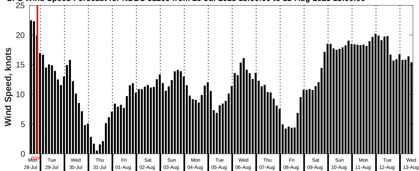
GFS Wind Speed Forecast for NDBC 51209 from 28-Jul-2025 13:00:00 to 13-Aug-2025 13:00:00
