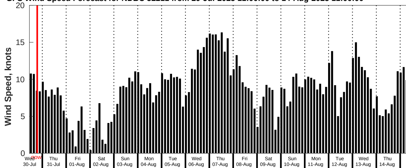
GFS Wind Speed Forecast for NDBC 52211 from 29-Jul-2025 11:00:00 to 14-Aug-2025 11:00:00
