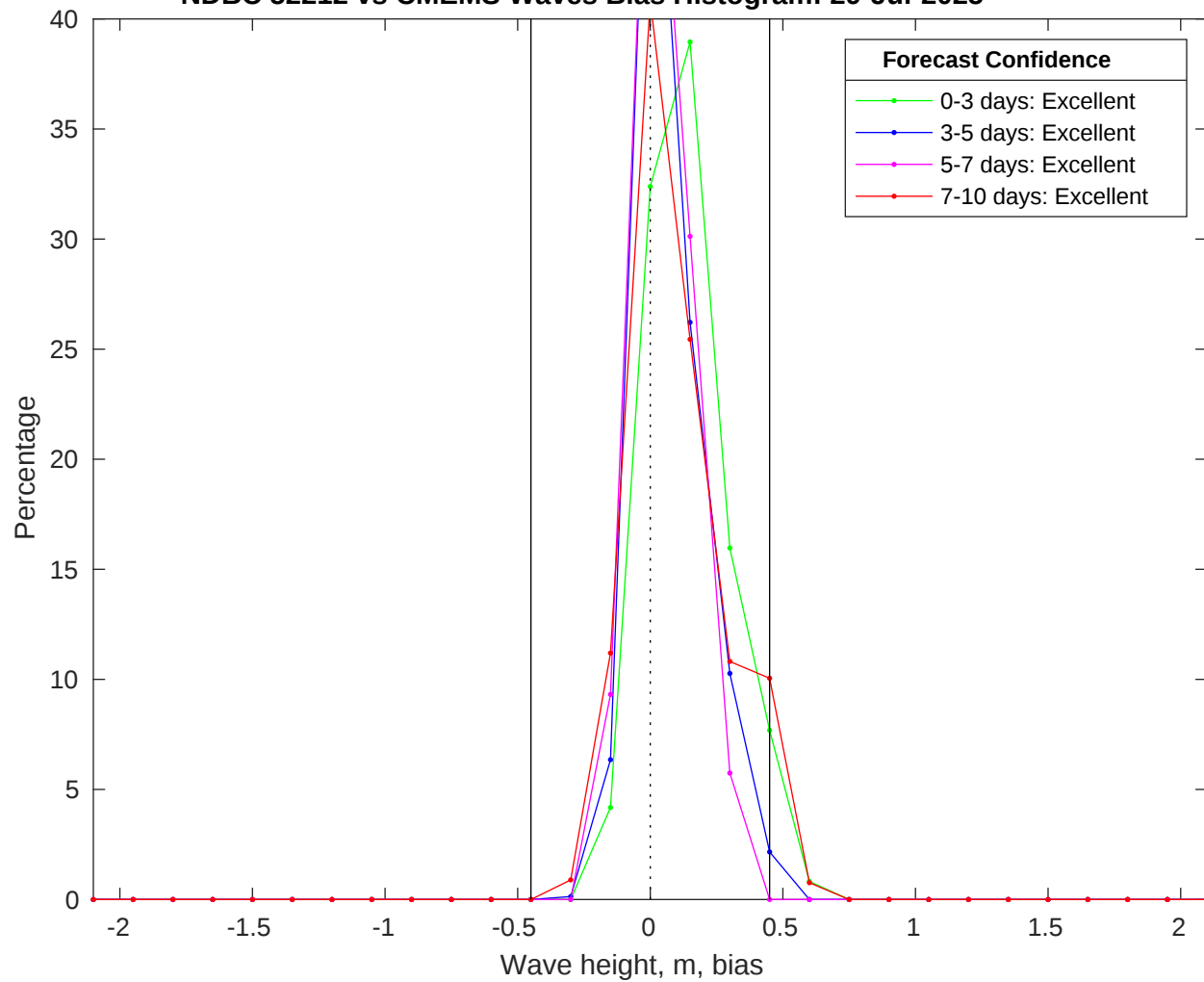
NDBC 52212 vs CMEMS Waves Bias Histogram: 29-Jul-2025
