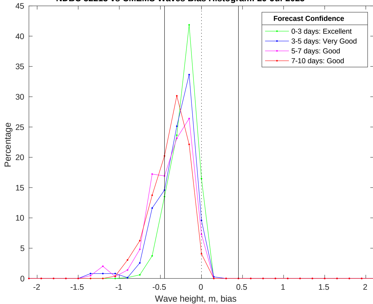
NDBC 52213 vs CMEMS Waves Bias Histogram: 29-Jul-2025
