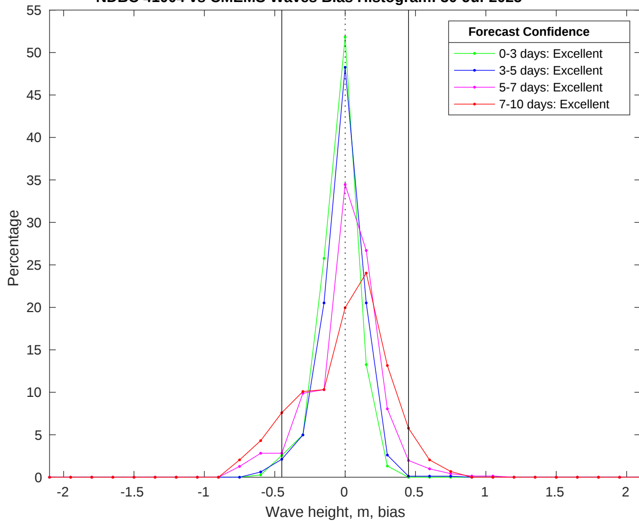
NDBC 41004 vs CMEMS Waves Bias Histogram: 30-Jul-2025
