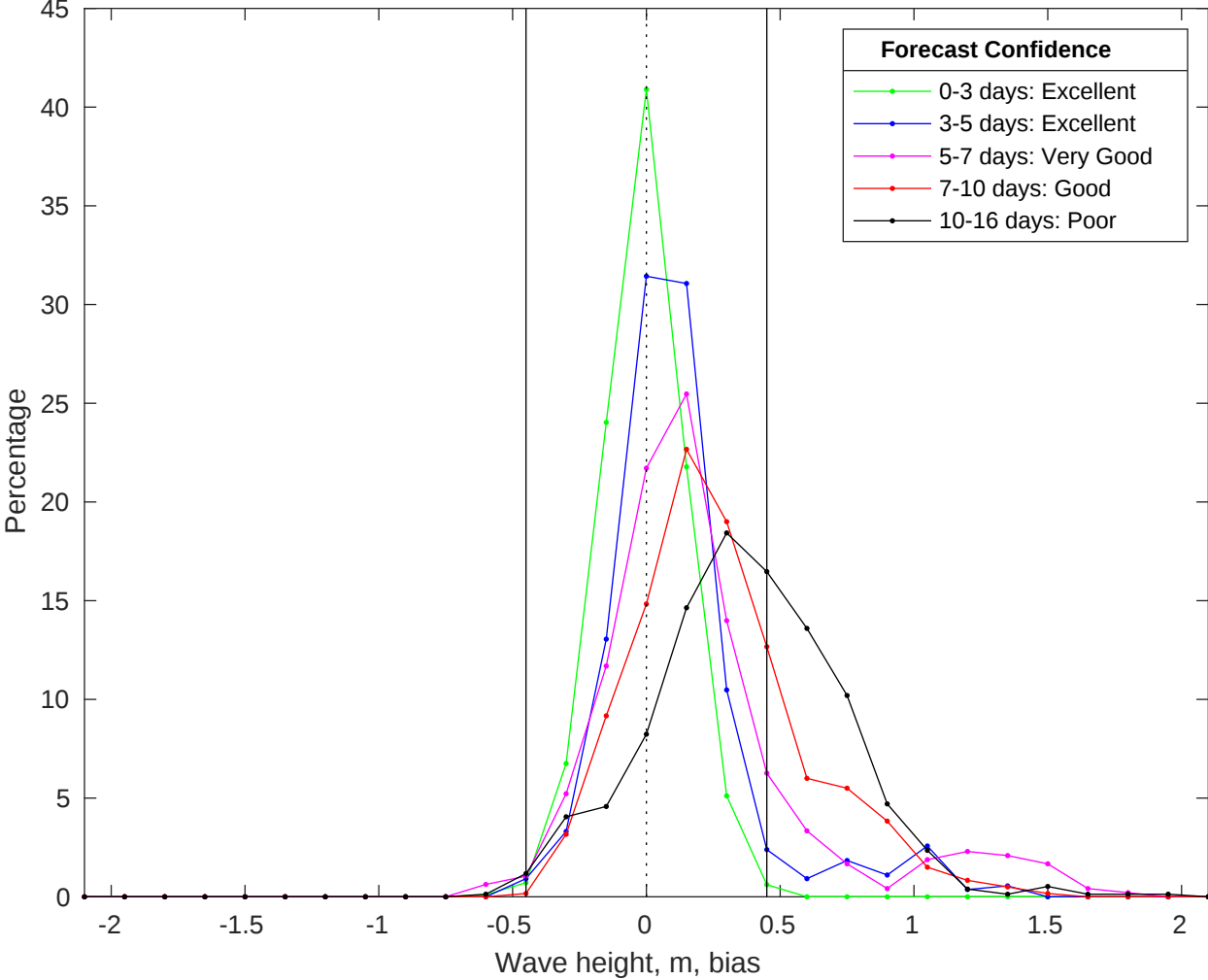
NDBC 41004 vs GFS Waves Bias Histogram: 30-Jul-2025
