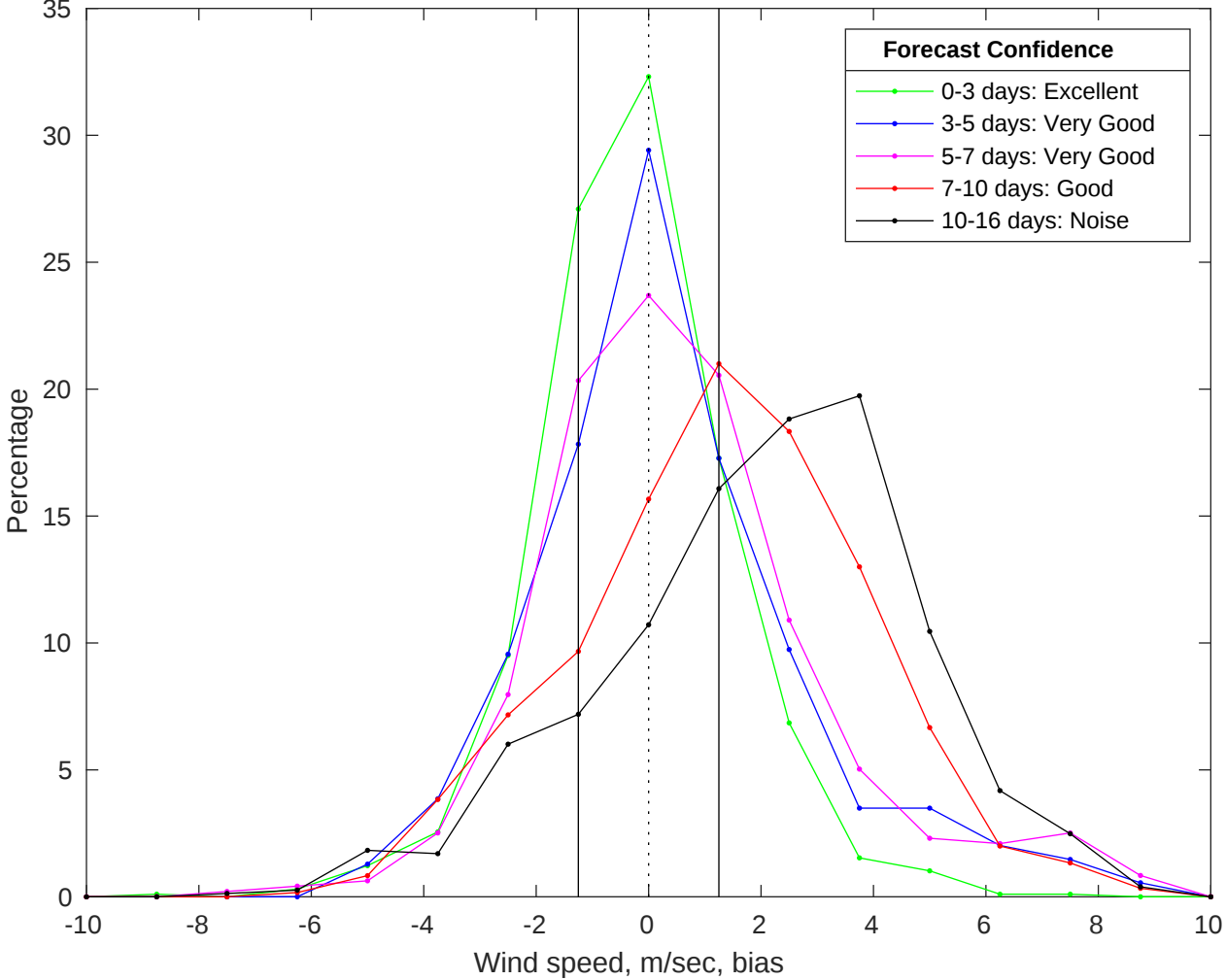
NDBC 41004 vs GFS Winds Bias Histogram: 30-Jul-2025
